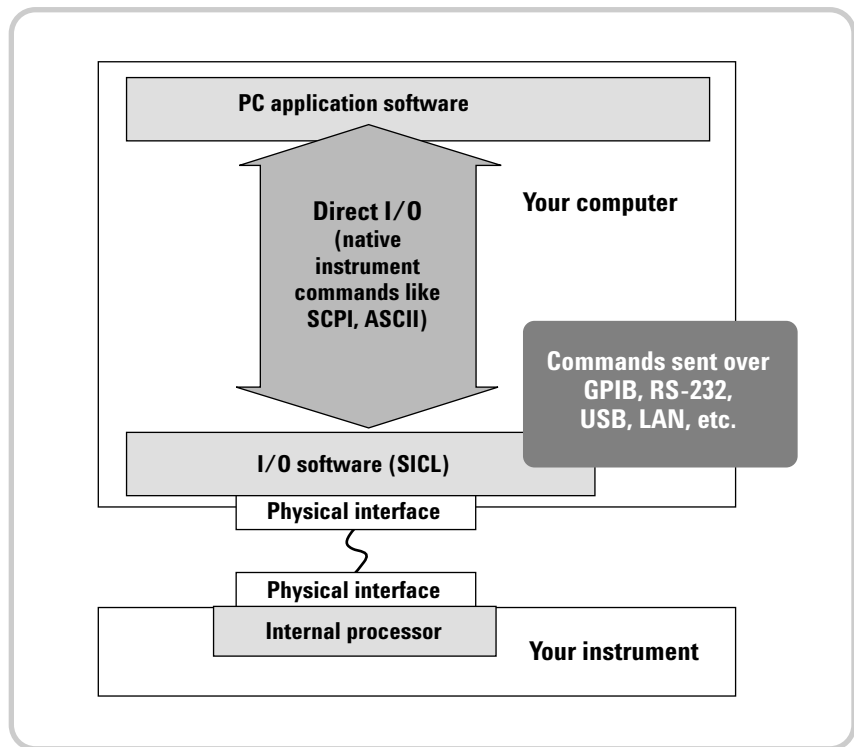
Figure 3. SICL I/O software reduces a test engineer's programming burden by making it easier to change I/O types (USB, GPIB, USB, VXI, RS-232, etc) without recoding the program. SICL adds a software layer, which has a small effect on system speed.
