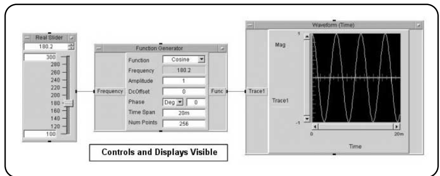
Figure 7. A tiny but interesting program, written in VEE. With its intuitive interface, VEE is the fastest T&M graphical language to learn. Fill in the boxes, and the VEE panel driver generates code for you. See http://we.home.agilent.com/upload/cmc_upload/tmo/downloads/E206HPVEE_TESTENGR_EVAL.pdf
